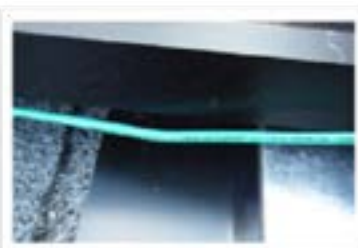
Photo 8: Source circuit conductors in contact with roof: NEC 338.10, 334.30
