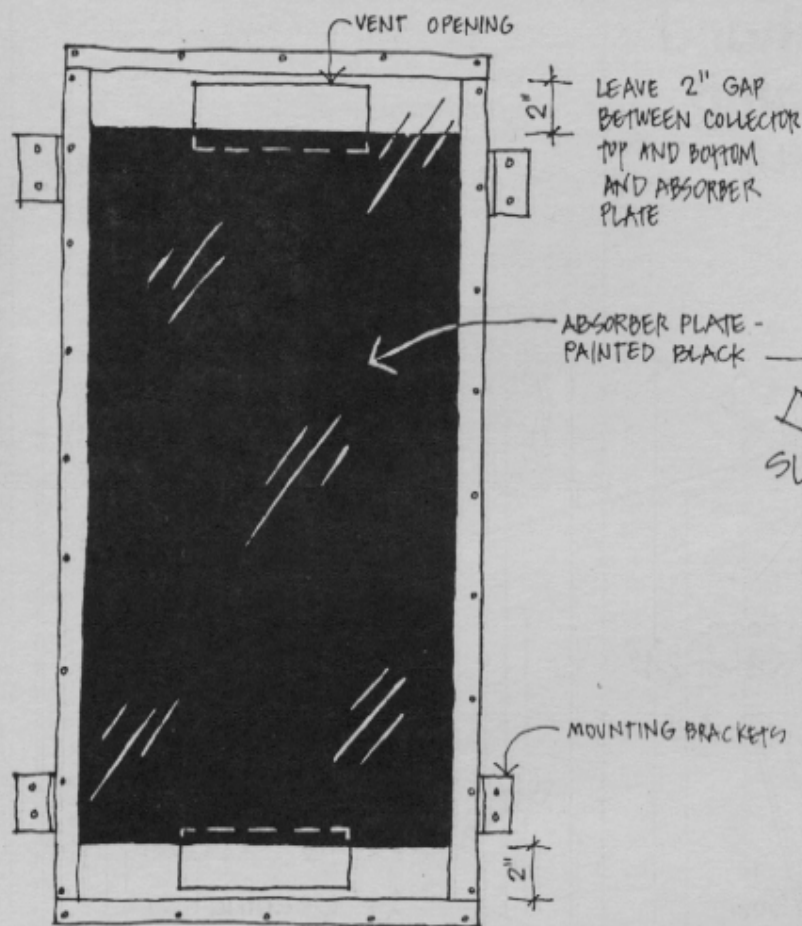
FRONT ELEVATION
